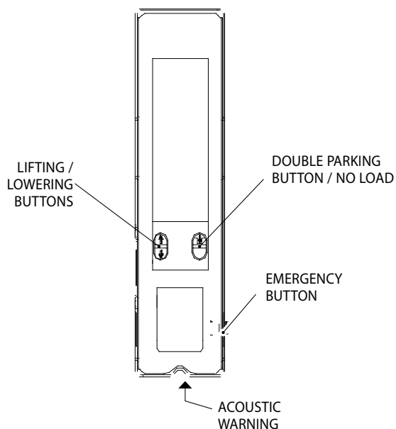
Electrical system part no. 049803240
