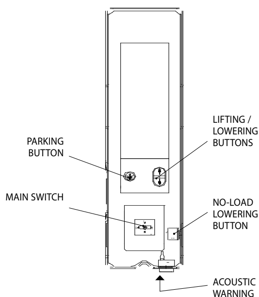
Electrical system part no. 049803021 049803030
