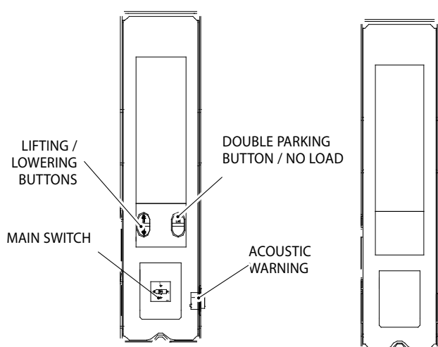
Electrical system part no. 049803210 049803220
