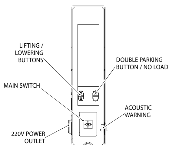
Electrical system part no. 049803230
