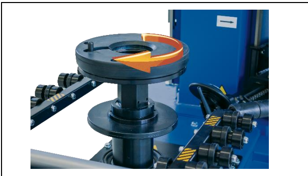
Tyre-changer-G1250.30_Floating plate-DI-4
